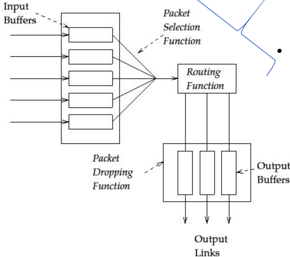
Figure 1: Basic Router Architecture
